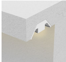
Detail B Terminating End with End Cap (STL6600-ECR)
