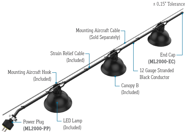
Canopy B (ML2000-CB)
