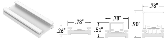
Mounting Channel (Dry or Wet Location) (LPL8150-UC)
