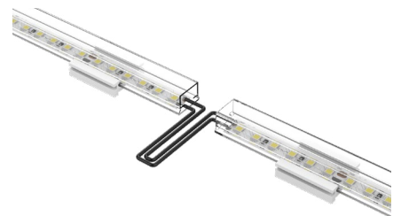
Detail C Continuous Connection (Wet Location)
