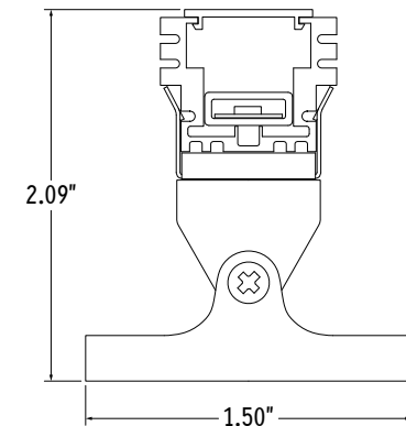
Assembled End View
