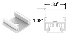
Surface Mounting Clip (LLED8400-SQL-MC)
