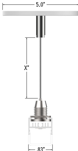
Pendant Mount (Pictured with Canopy) (LLED8400-SQL-PM-X) (X = Specify Length)
