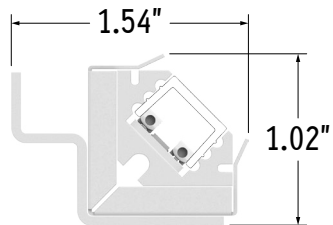
Assembled End View
