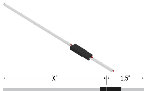
Power Connector White (20/2 Gauge Wire with White Jacket) LLED8050-CC-WH (33" Standard) LLED8050-CC-WH-X (X = Specify Length)
