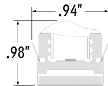
Asymmetric Lens
