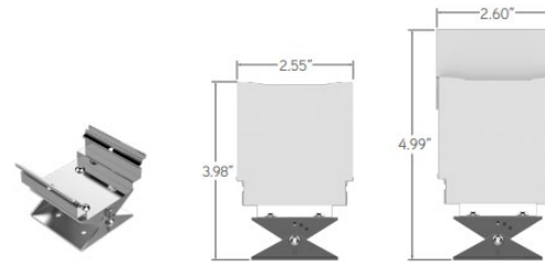
Mounting Clip (Adjustable with Locking Mechanism) (ALS600T-MC-3)
