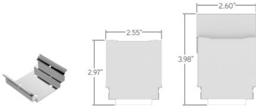
Mounting Clip (ALS600T-MC)
