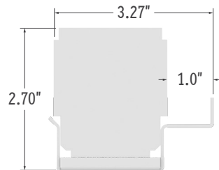
Assembled End Views
