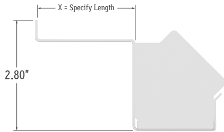
Assembled End Views
