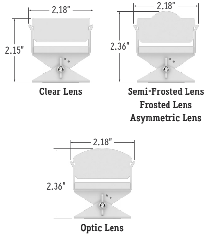
Assembled End Views
